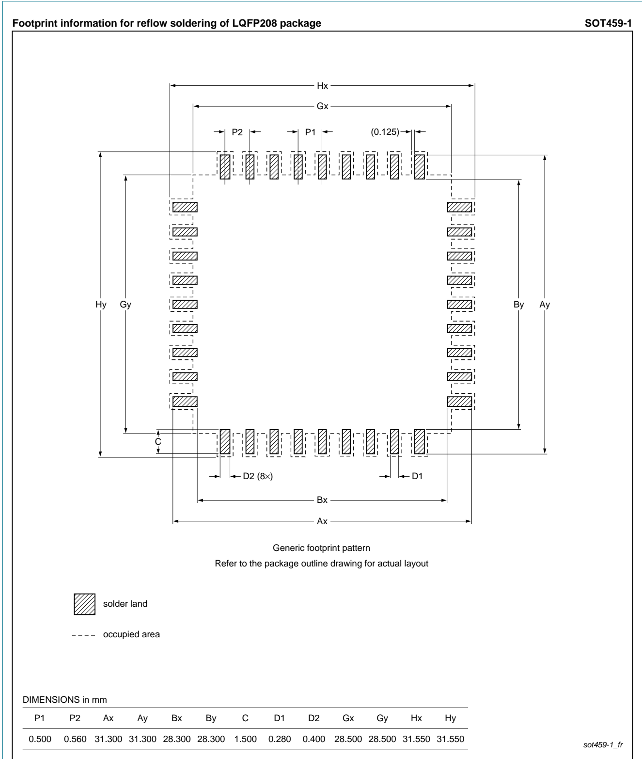
Fig 52. Reflow soldering of the LQFP208 package
