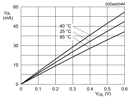
Fig 20. High-drive pins; typical LOW level output current I_{OL} versus LOW level output voltage V_{OL}
