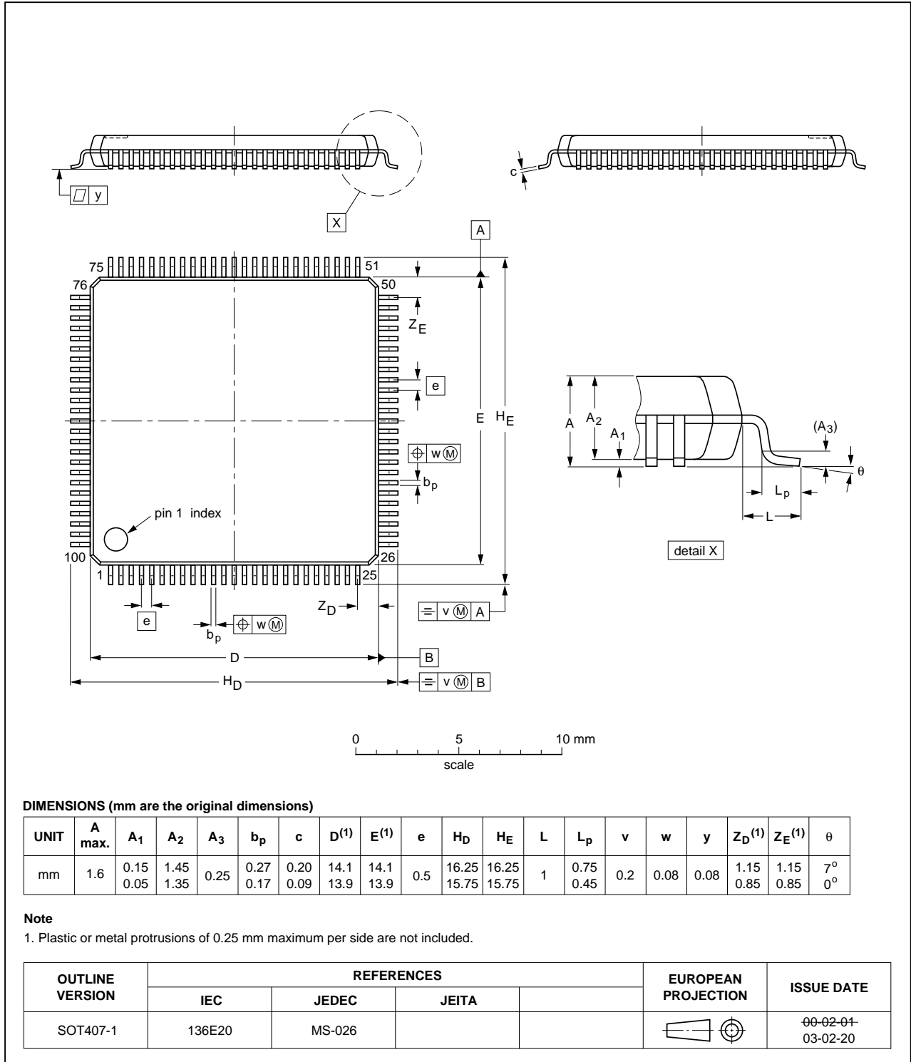
Fig 49. Package outline for the LQFP100 package
