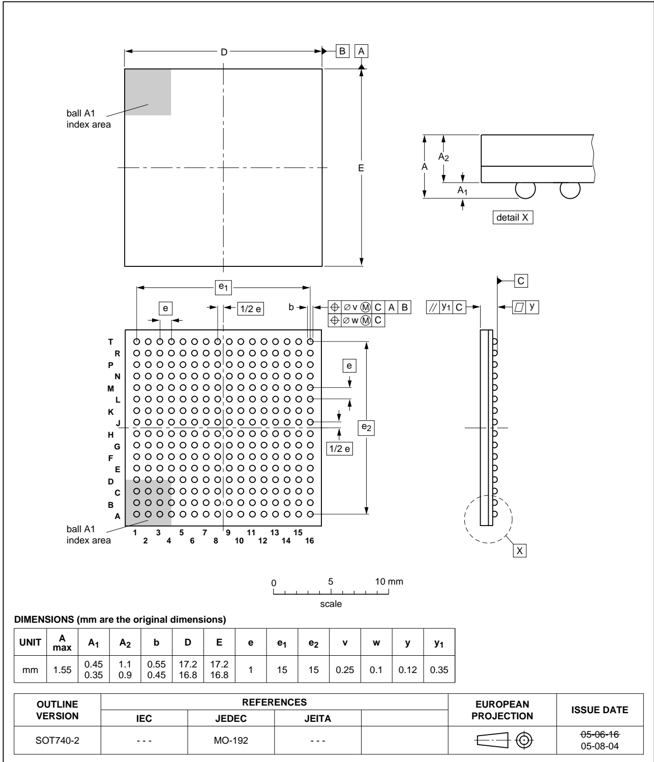
Fig 44. Package outline of the LPGA256 package
