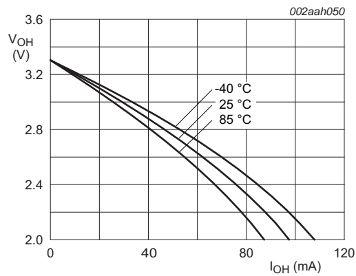
Fig 21. High-drive pins; typical HIGH level output voltage V_{OH} versus HIGH level output current I_{OH}
