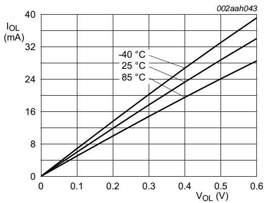
Fig 20. High-drive pins; typical LOW level output current I_{OL} versus LOW level output voltage V_{OL}
