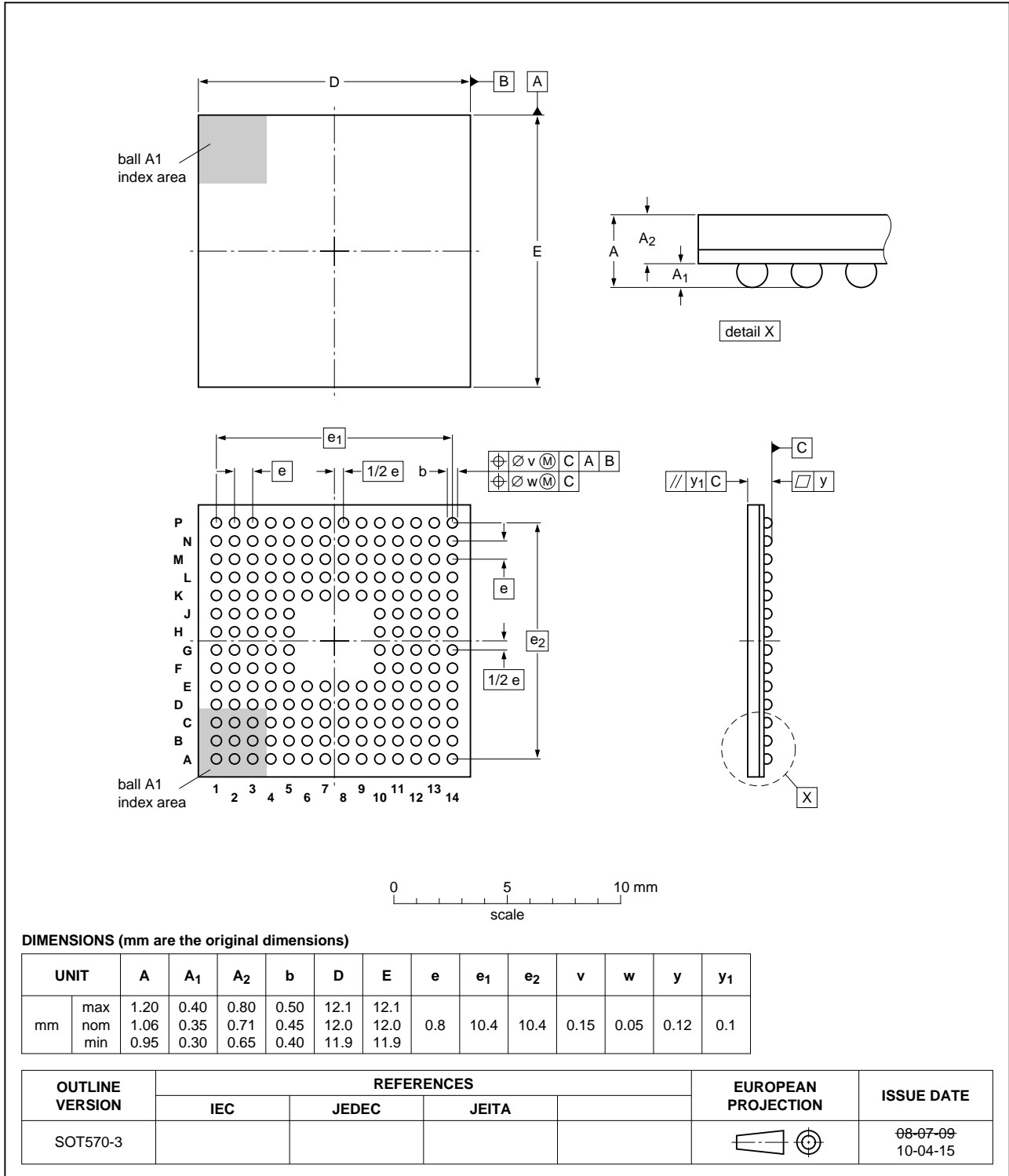
Fig 45. Package outline of the TFBGA180 package
