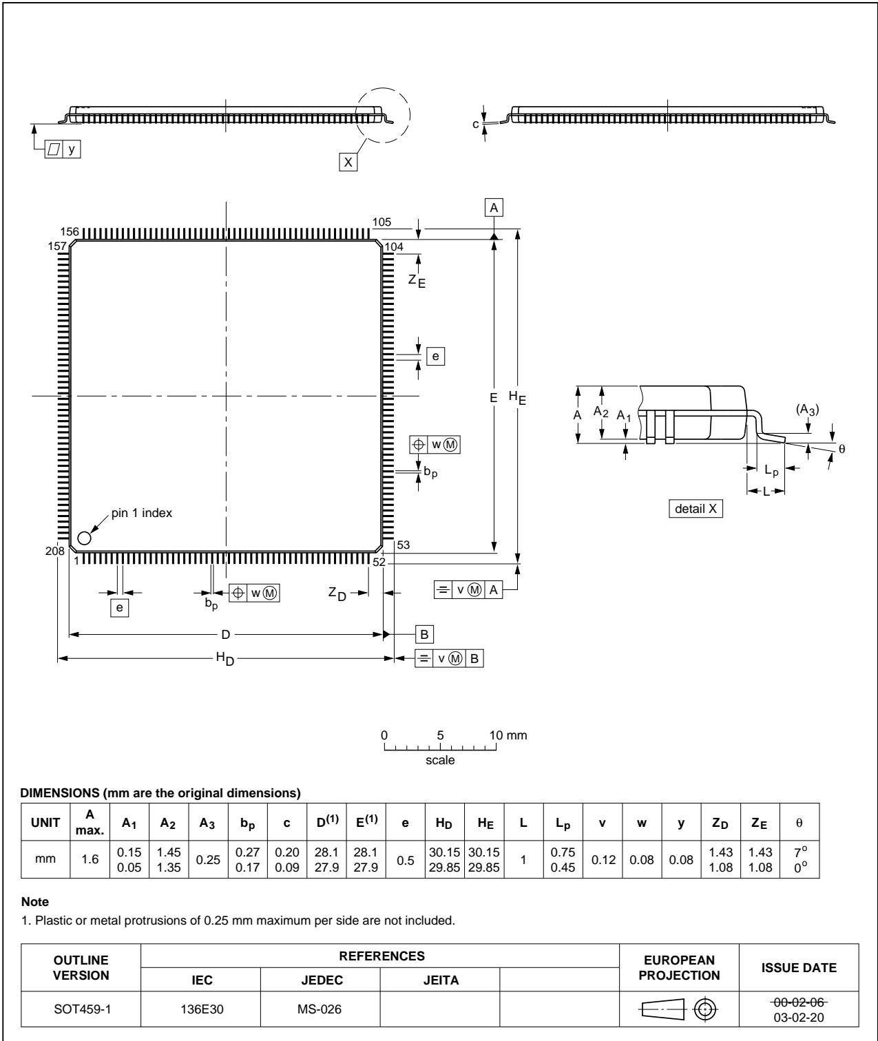
Fig 46. Package outline of the LQFP208 package
